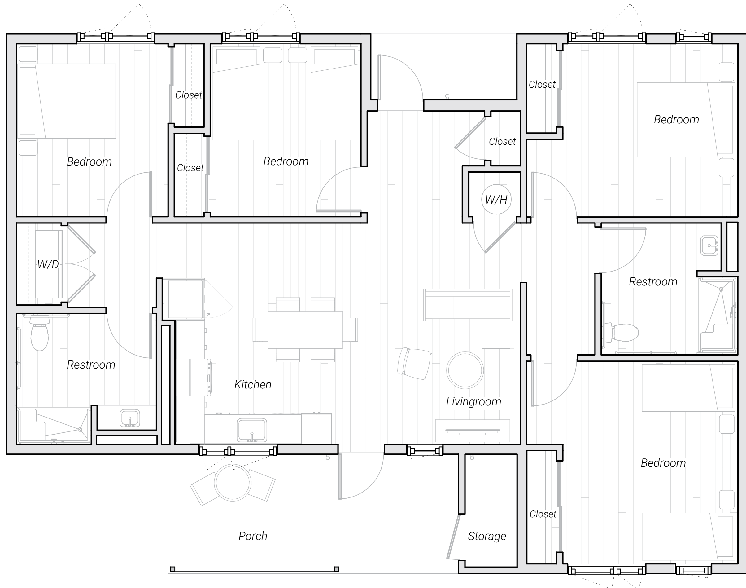
4 Bedroom - ADA Accessible Area 1,515 sf
