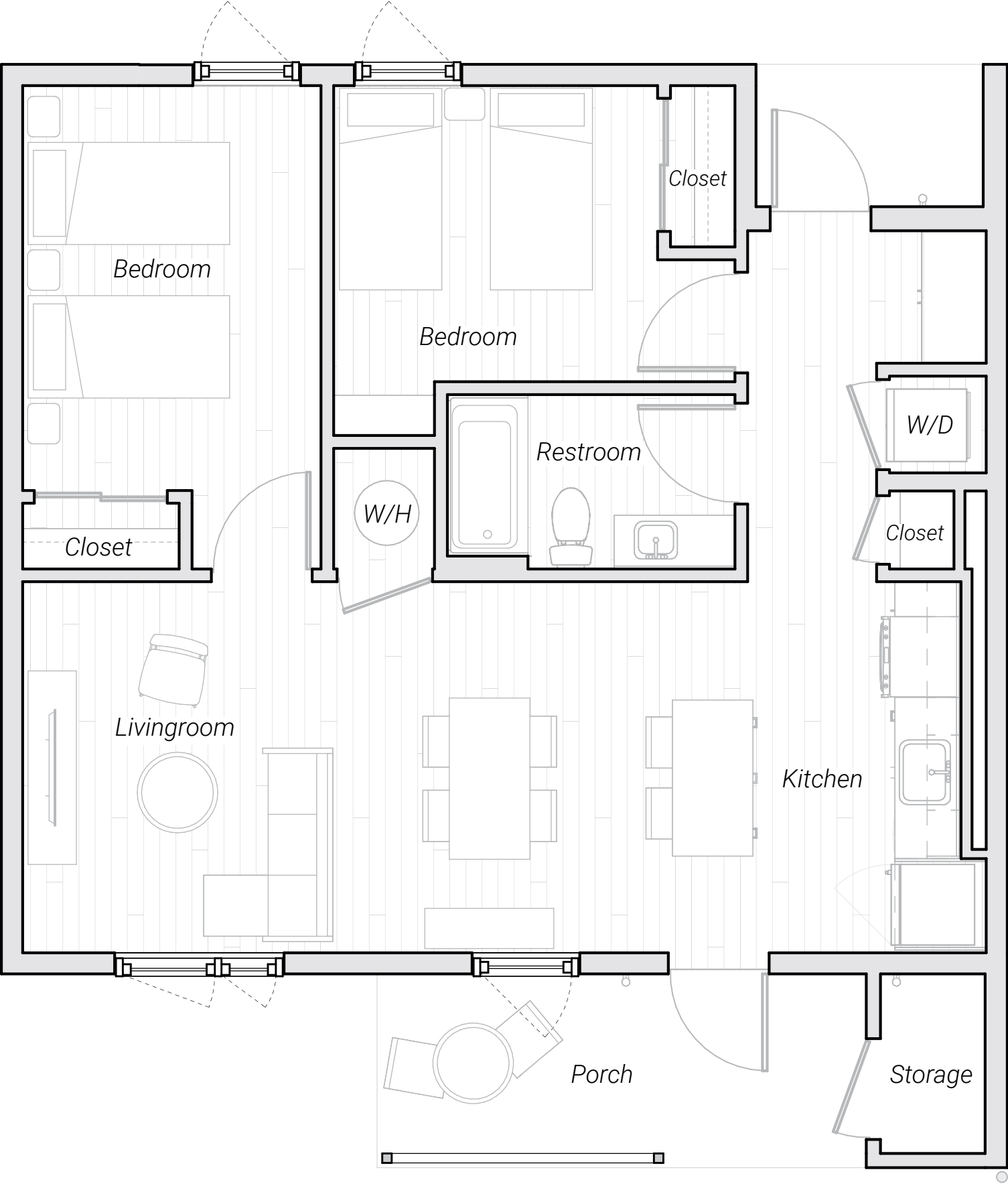
2 Bedroom Area 869 sf
