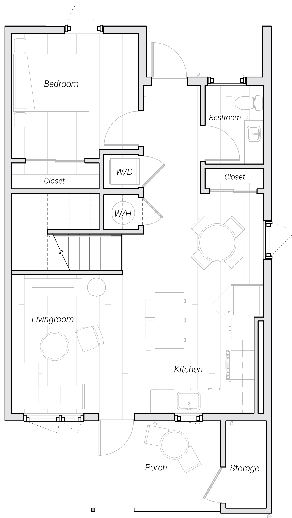
3 Bedroom - Level 01 Area 1,298 sf
