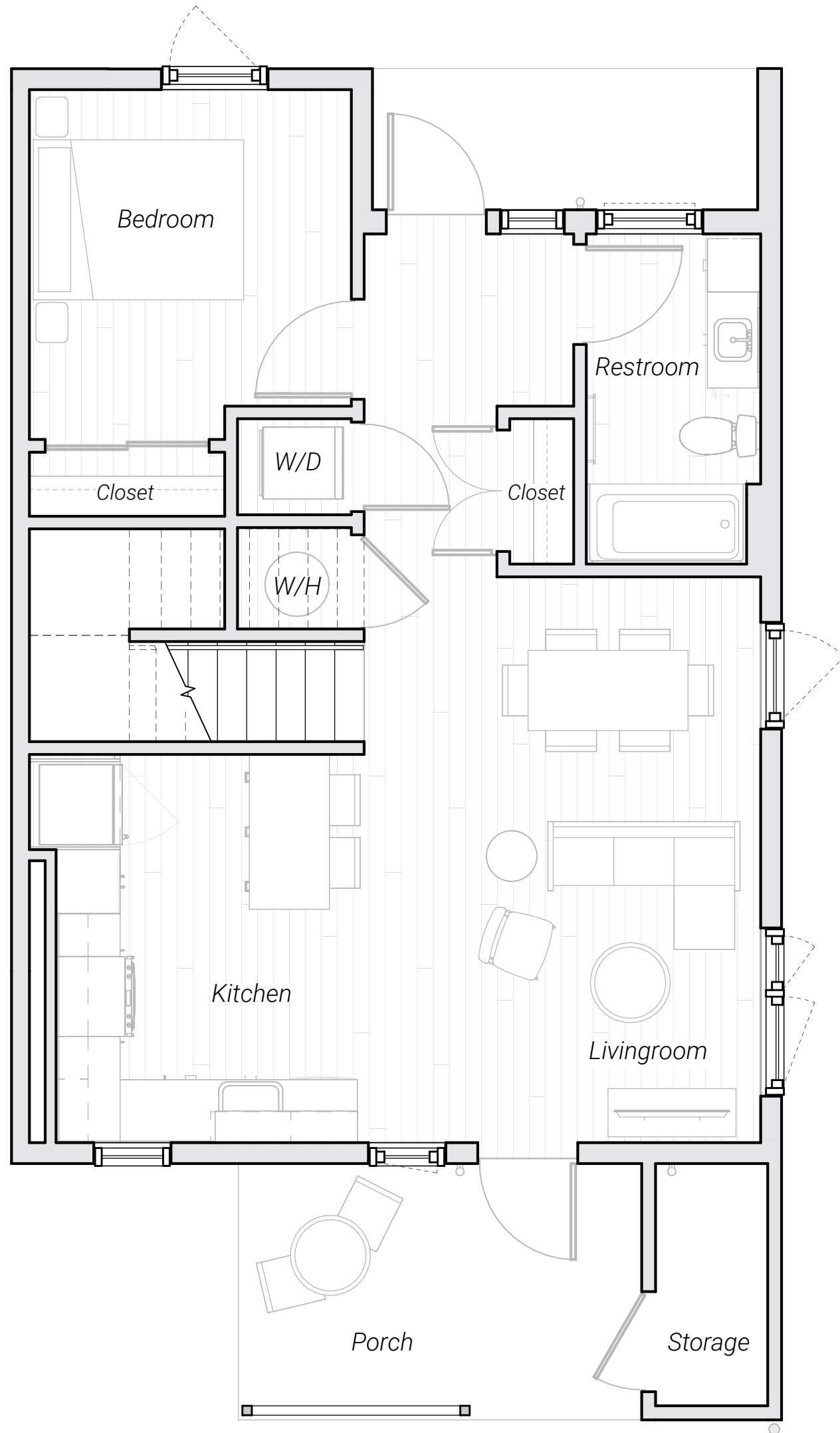
4 Bedroom - Level 01
