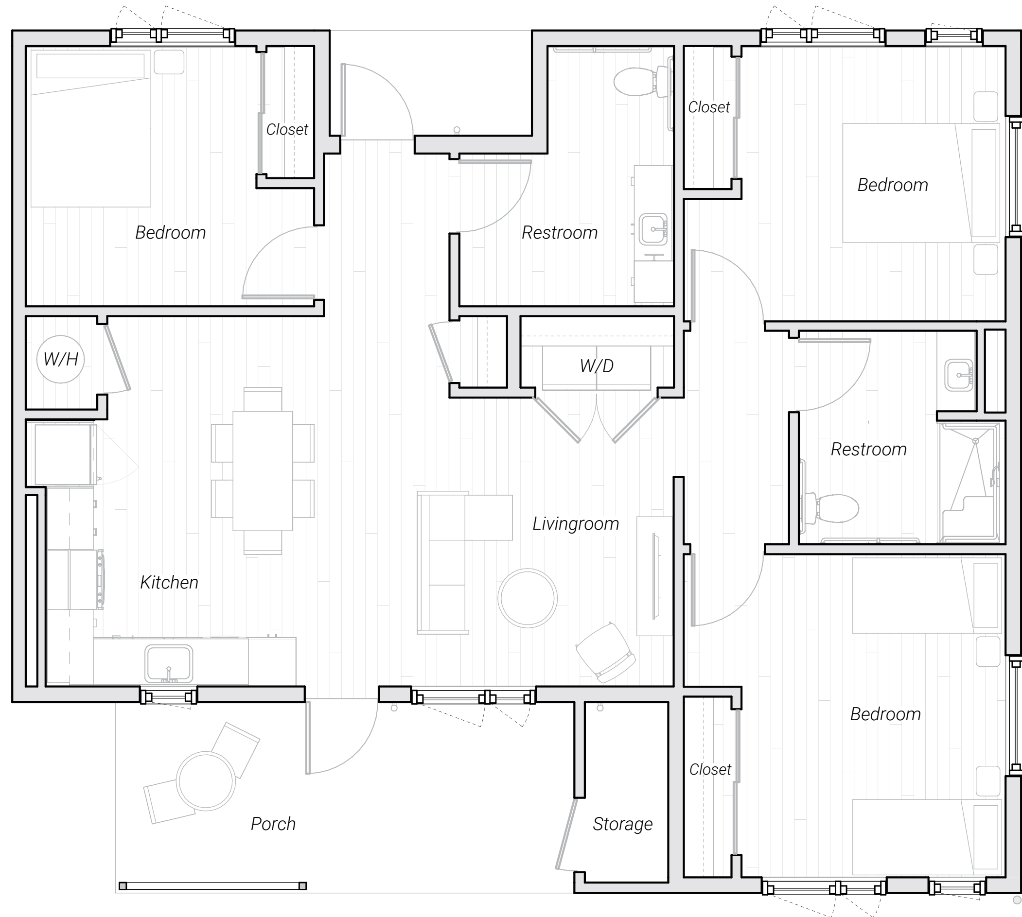
3 Bedroom - ADA Accessible Area 1,310 sf
